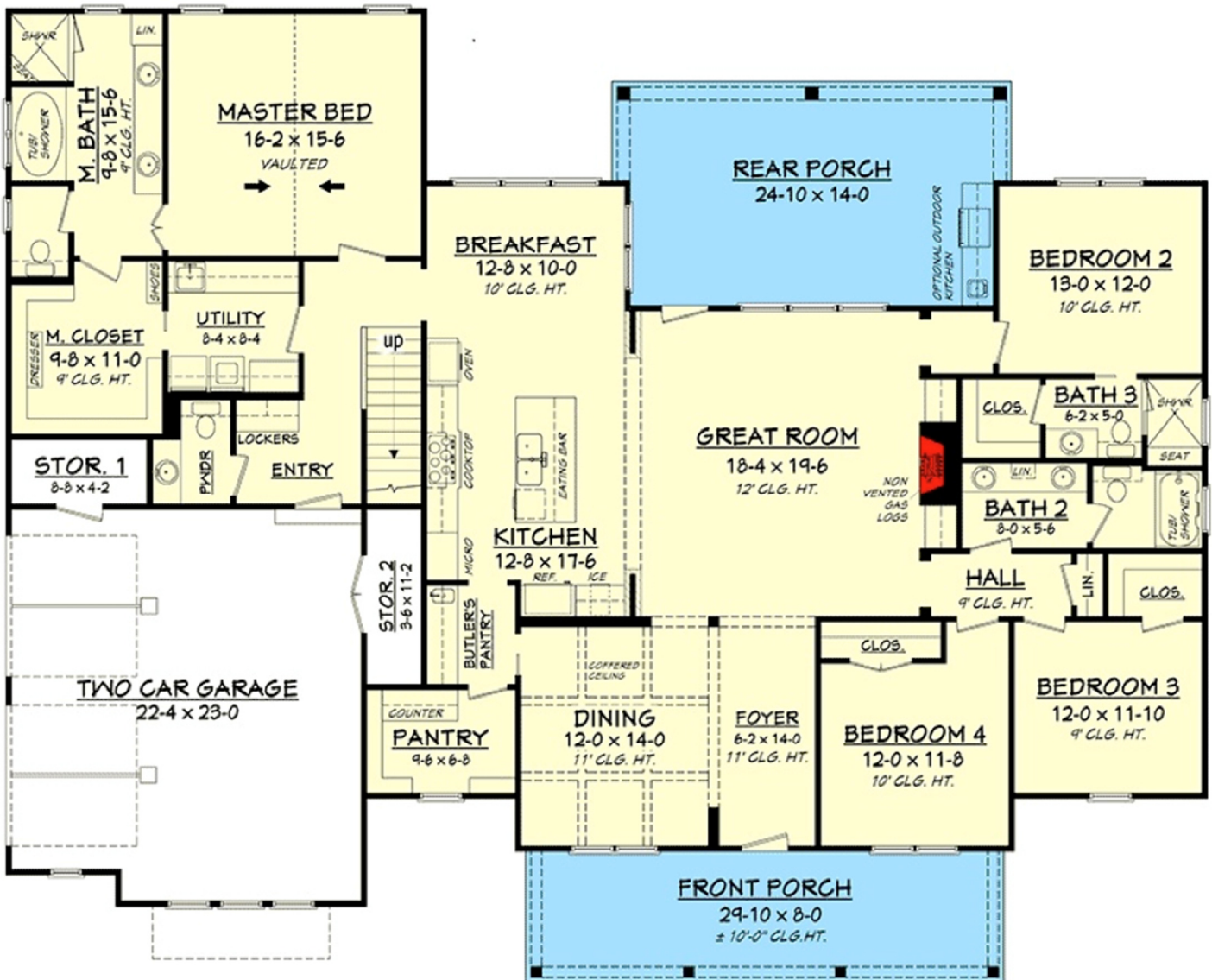
First Floor
