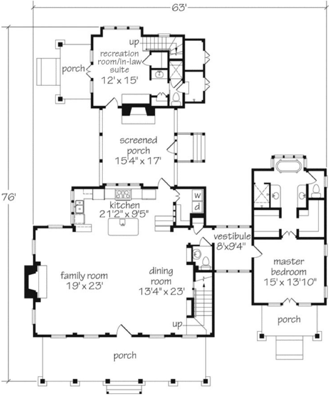
First Floor
